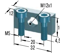
MB12SC2 *€ 14,23 Montageblock
