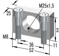
MB25SC2-V4A *€ 38,80 Montageblock
