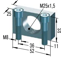
MB25SC2 *€ 25,04 Montageblock
