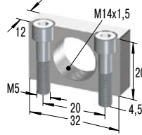
MB14SC2-V4A *€ 28,14 Montageblock
