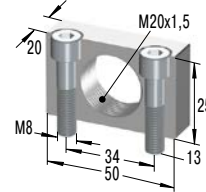
MB20SC2-V4A *€ 31,15 Montageblock
