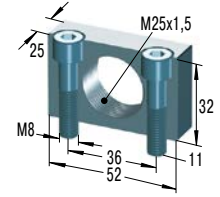
MB25SC2 *€ 25,04 Montageblock
