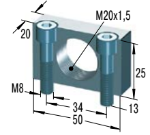
MB20SC2 *€ 17,62 Montageblock
